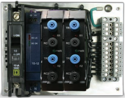
Retro Kit Open Assembly
