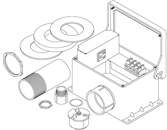
(Standard 10A600 Caddy Box Shown)
